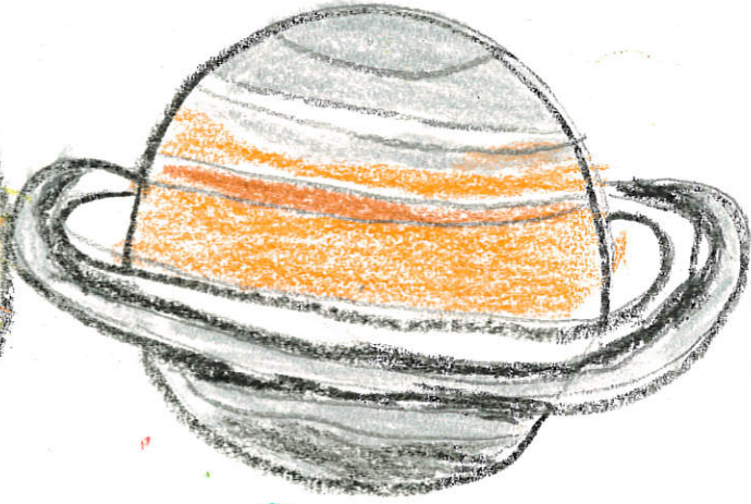
Saturn
